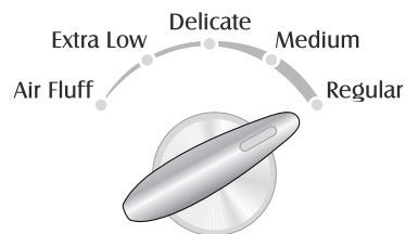
Infinite Temperature
